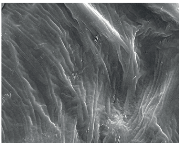
Scanning Electron Microscopy (SEM) image of the micromorphology of Arabidopsis thaliana leaves covered with an epicuticular wax sheath.
